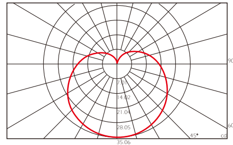
Light Distribution Curve (cd) - Daylight
