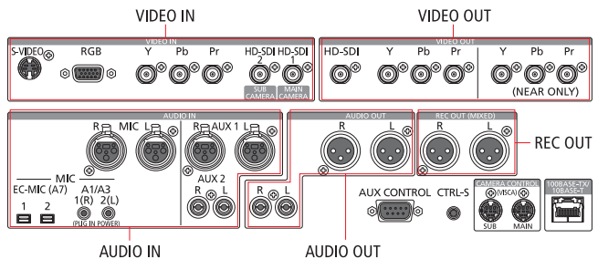
Rear Panel
