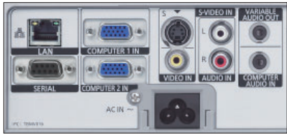
NOTE: The photo shows the rear terminals for the PT-LB90NTEA.
