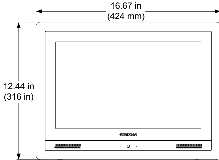
Overall Dimensions (V15-WALL Front View - With Bezel)
