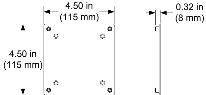
Overall Dimensions (VESA Mounting Bracket - Front and Side View)
