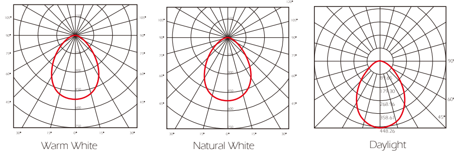
Light Distribution Curve (cd)
